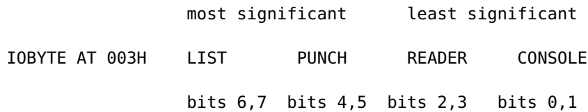
Figure 6-1. IOBYTE Fields
